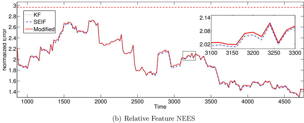
Figure 3-3: The relative normalized estimation error squared (NEES) for the (a) vehicle and (b) a representative feature based upon the same series of Monte Carlo simulations that we use to calculate the global error. We compute the relative error by transforming the original random vector with respect to the first feature instantiated in the map: \xi_{m_1 i} = \ominus \mathbf{m}_1 \oplus \xi_i . Both plots include a horizontal line that denotes the 97.5% chi-square upper bound. The relative map error for both the SEIF and modified rule is nearly identical to that of the KF, suggesting that the SEIF preserves the relative consistency of the state estimates.
